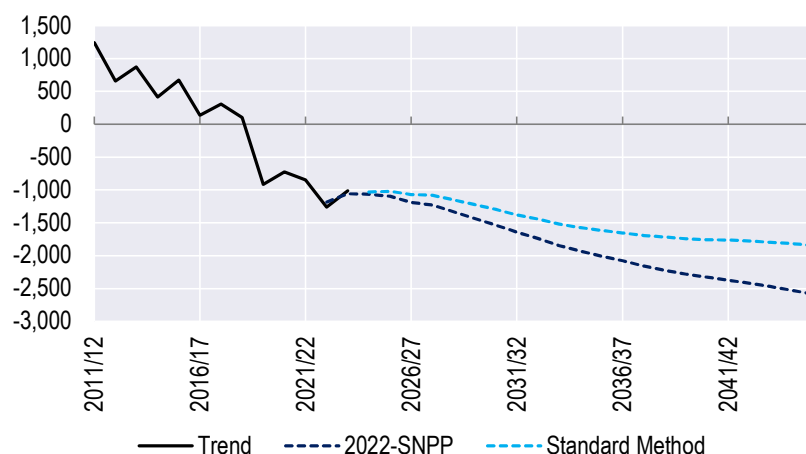
Figure 4-11: Past trends and projected natural change – Gloucestershire
