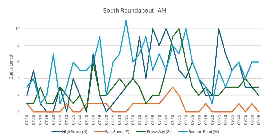
Figure 2-11: South roundabout (AM) - Queue length
