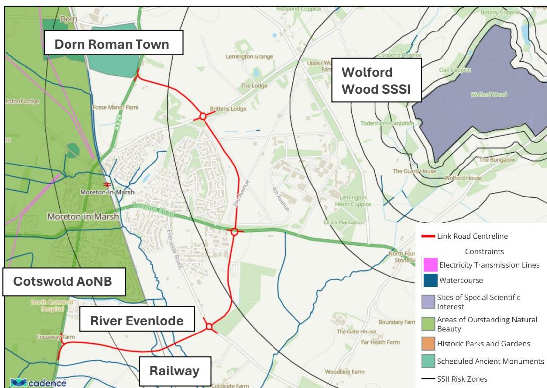
Figure 4-1 Link Road Physical Constraints
