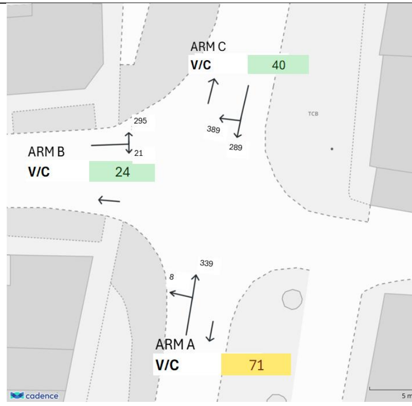
Figure 5-9: DS3 (PM) - Mini-roundabout performance
