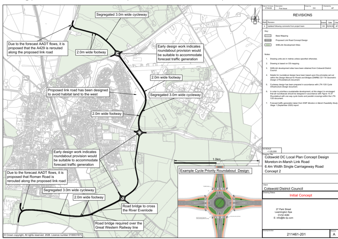
Figure 4-13 Concept Design
